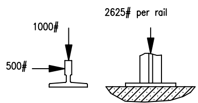
RAIL REACTIONS
