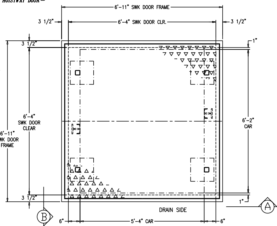
DETAIL 1
