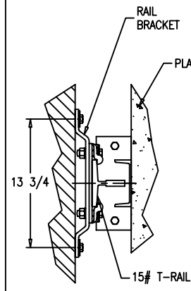
DETAIL 1
