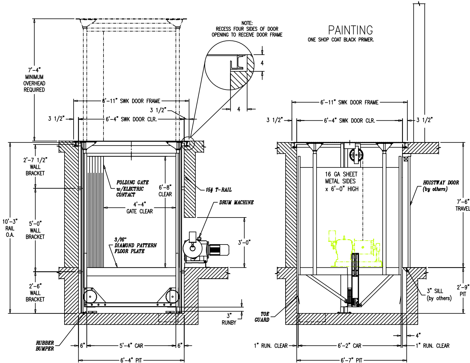
SECTION A
