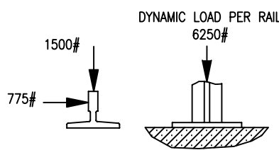
RAIL REACTIONS
